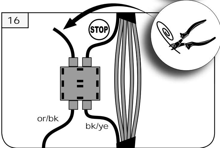
E-Satz or/bk → kabel bk/ye e-kit or/bk → cabel car bk/ye
