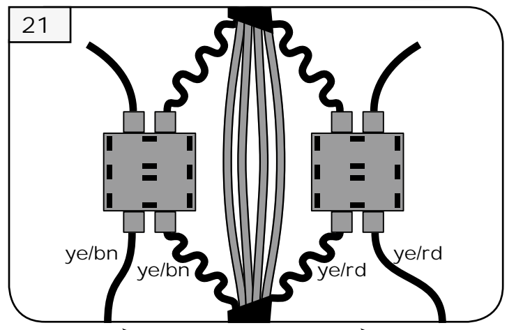
E-Satz ye/bn → kabel ye/bn, E-Satz ye/rd → kabel ye/rd e-kit ye/bn → cabel car ye/bn, e-kit ye/rd → cabel car ye/rd
