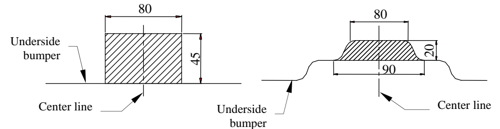
Fig. 2 Bumper cut out Ford Maverick
